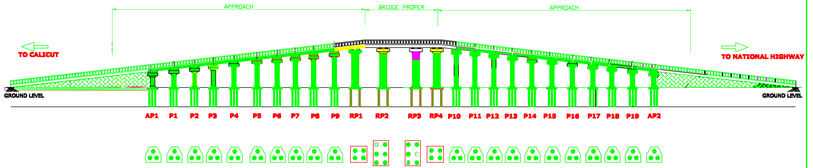
PILE FOUNDATION
