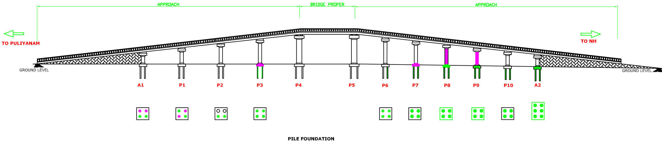
PILE FOUNDATION
