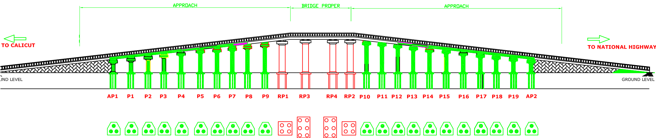
PILE FOUNDATION
