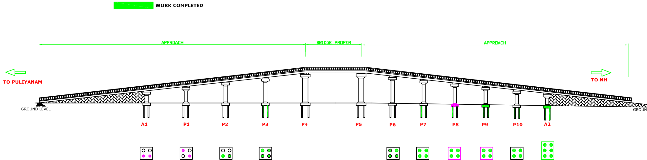
PILE FOUNDATION
