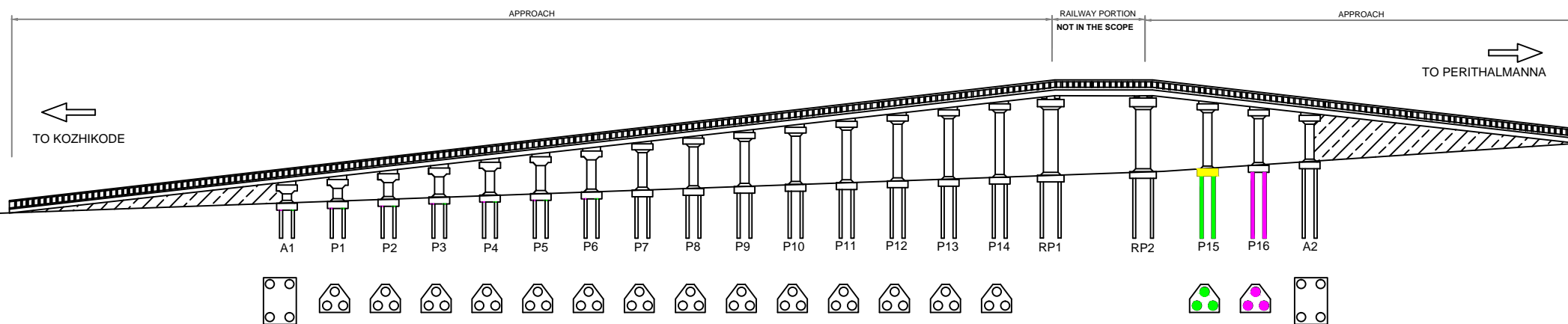
PILE FOUNDATION
