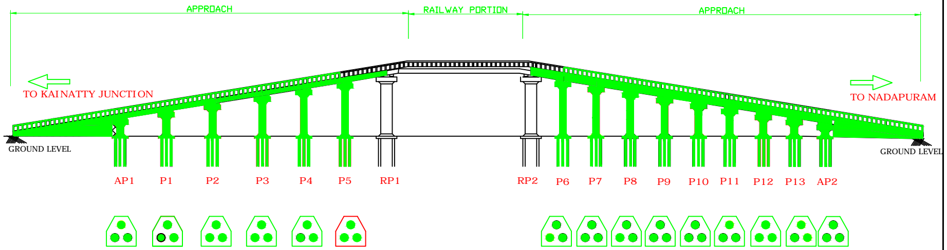
PILE FOUNDATION
