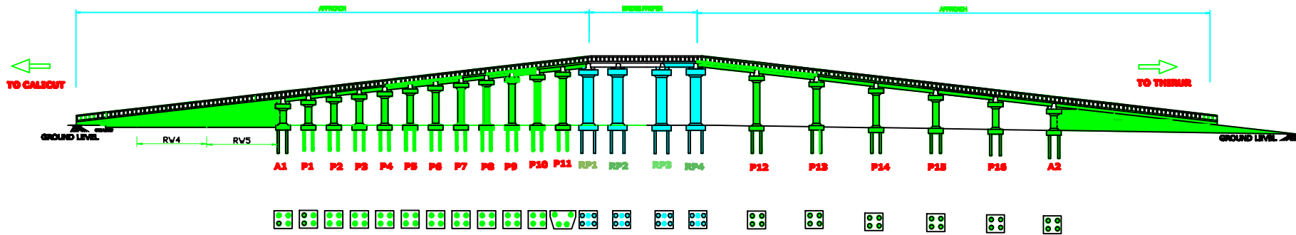
PILE FOUNDATION
