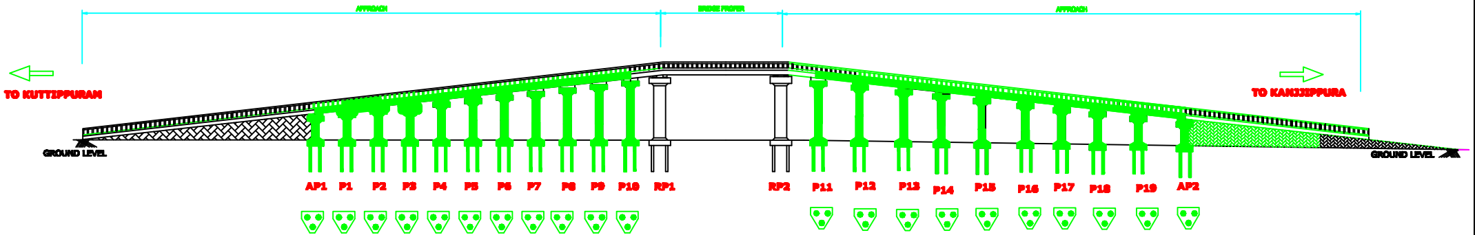
PILE FOUNDATION
